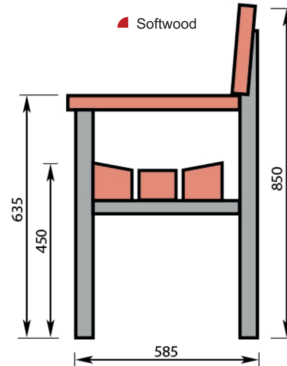
'Zurich' type timber seat
